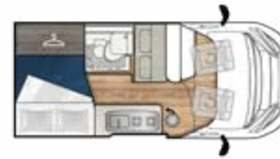
E-Van K2 Premium/Trend ↪ 5410 mm
